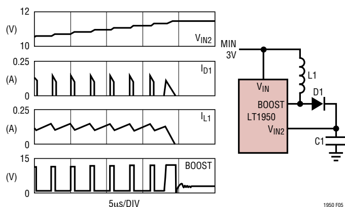
Figure 5. V_{IN2} Generation Using the BOOST Pin
